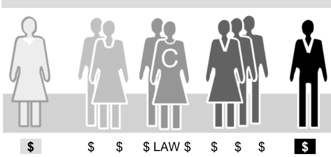
Fair shares give minority voters some power.
